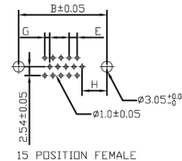
15 POSITION FEMALE
