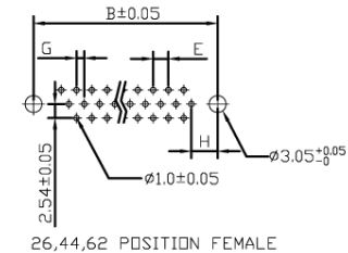
26,44,62 POSITION FEMALE
